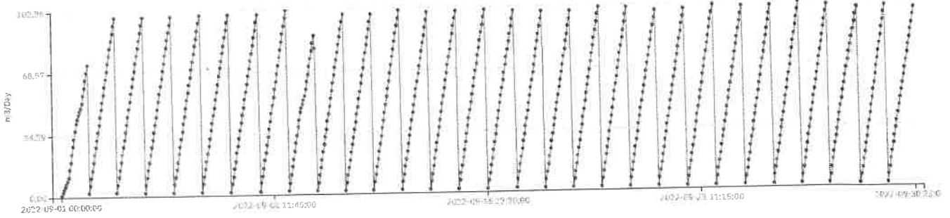
GW_1_BOREWELL_Inlet_flow-Totalizer Flow_Raw
